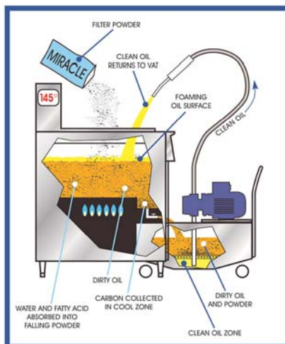
Wheel-up Filtering Machines
